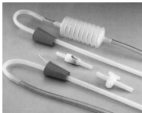
A-BELLOW; B-PUSH TAP; C-BUTTERFLY TAP
